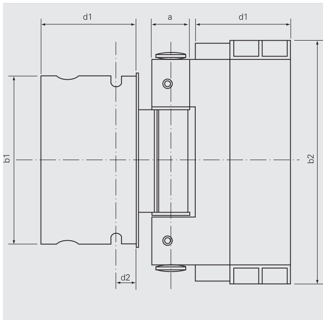
Application doppie gasket
