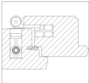
Application single gasket
