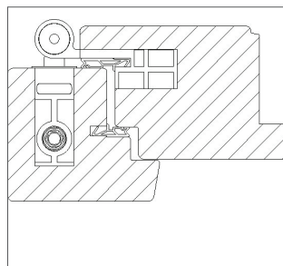
Application doppie gasket
